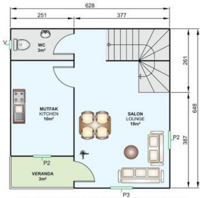
37 m 2 + 3 m 2 = 40 m 2 Zemin Kat Planı / Ground Floor Plan
