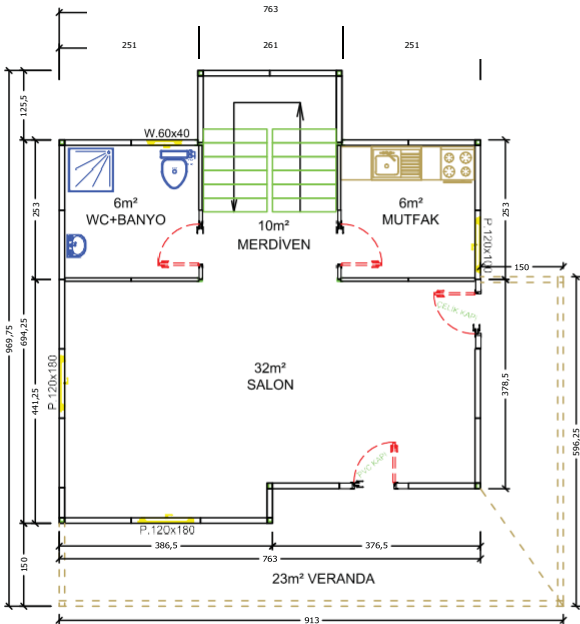
ZEMİN KAT: 54m 2 + 23m 2 = 77m 2
